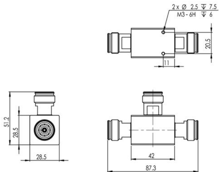
TPS8-43-555_6000_Drawing
