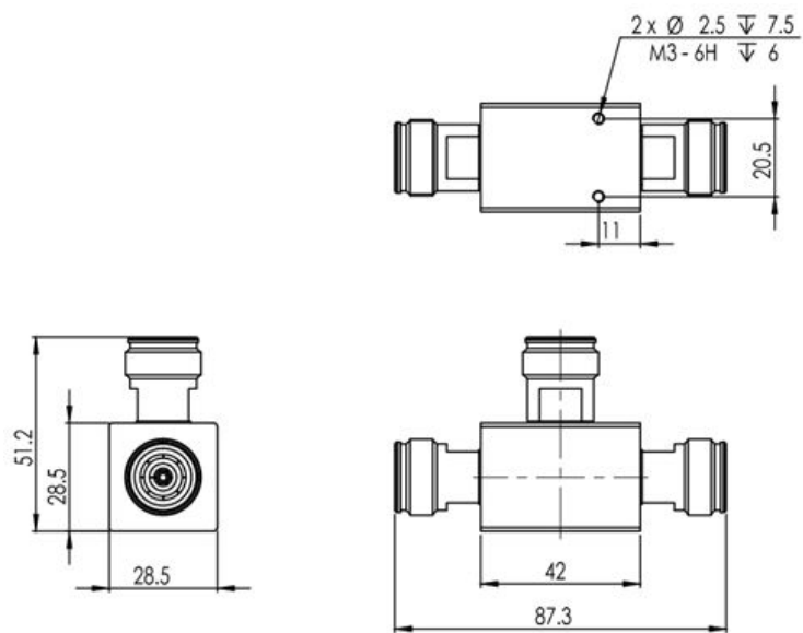
TPS6-43-555_6000_Drawing
