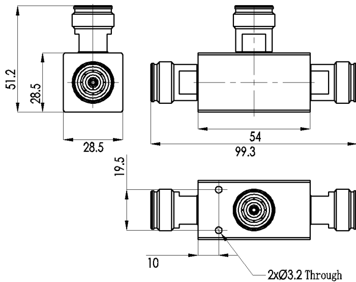
Outline Drawing
