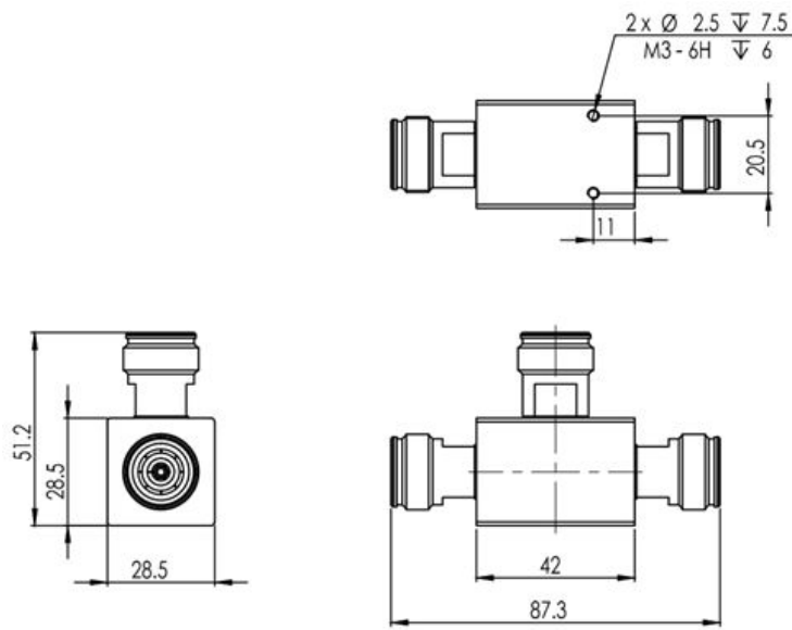
TPS10-43-555_6000_Drawing
