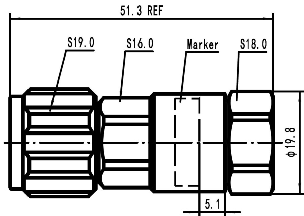
NM-SCF12-C03 Outline Drawing
