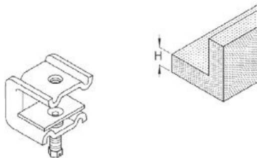
Installation Example
