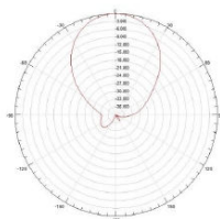
1695-2690MHz Vertical
