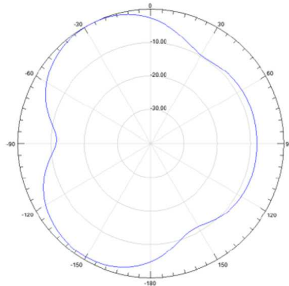
Vertical Pattern
