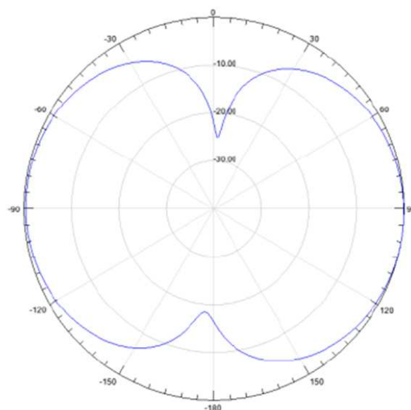
Vertical Pattern
