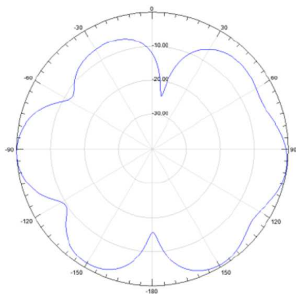
Horizontal Pattern
