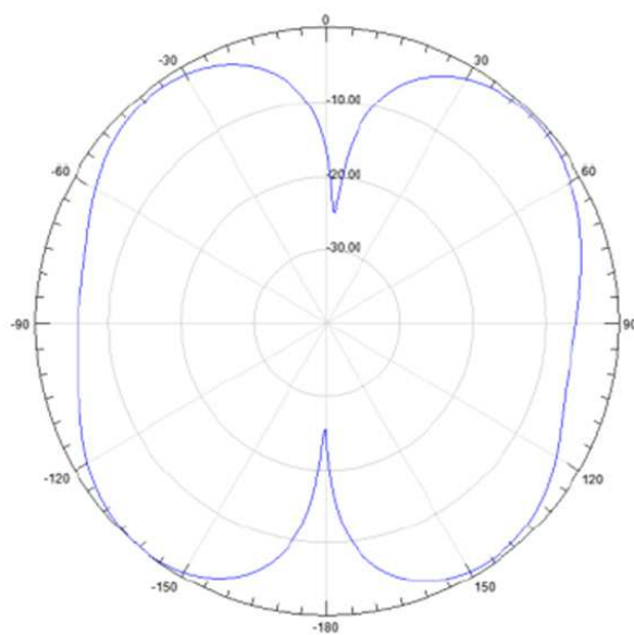
Horizontal Pattern
