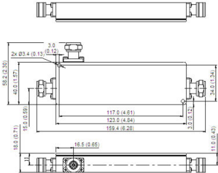
Dimensions mm(inch)
