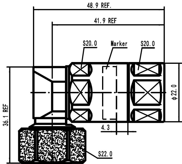
43MR-LCF12-C03 Outline drawing
