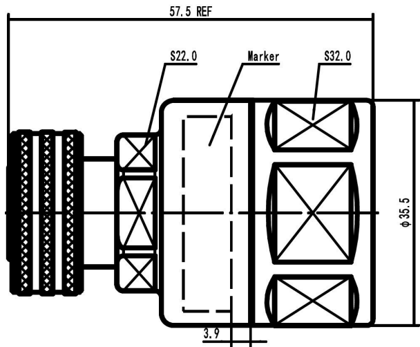
43MP-LCF78-C03 Outline drawing
