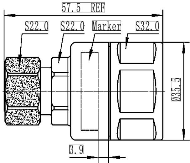
43M-LCF78-C03 Outline Drawing
