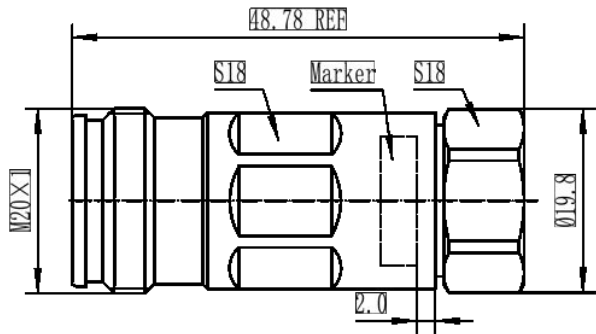
43F-SCF12-C03 Outline Drawing
