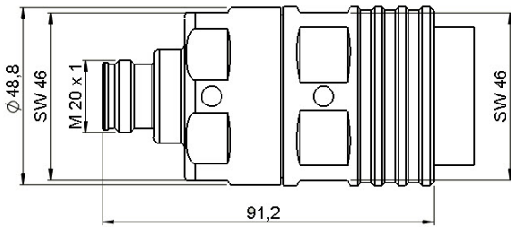
43F-RA114-P02 sketch
