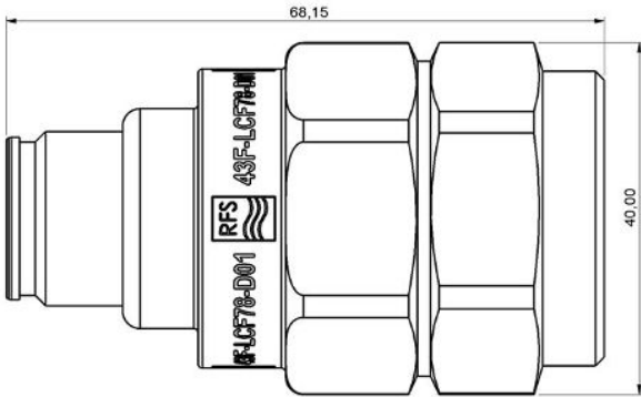
43F-LCF78-D01 Outline Drawing
