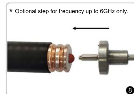
Use the shaping tool to insert the sealed ball into the inner conductor. The ball is below the inner conductor more than 20mm.
