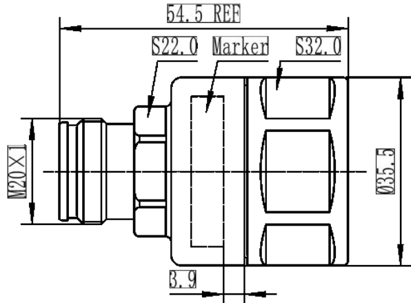
43F-LCF78-C03 Outline Drawing
