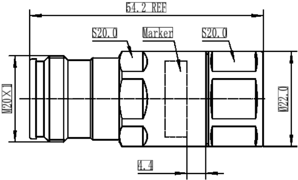
43F-LCF12-C03 Outline Drawing
