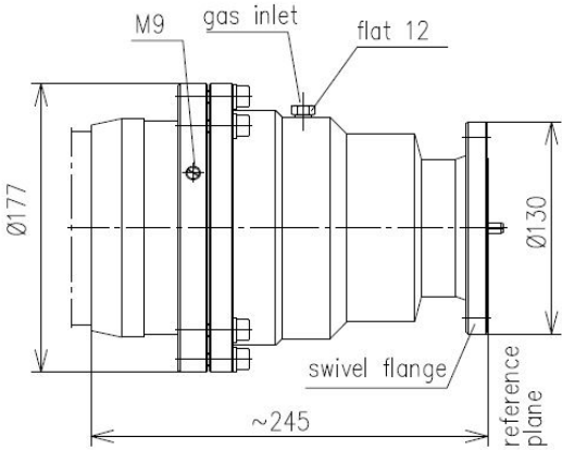
318EIA-HCA495_DRW
