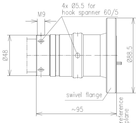
158EIA-LCF114-062 (Dimensions are in mm)
